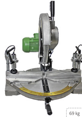
HA 1014 Portable Single Head Saw-Pneumatically Clamped
